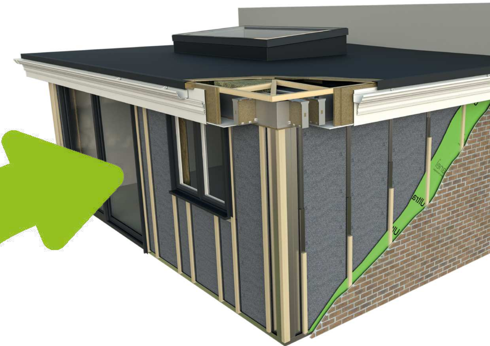
hup! Flat Roof with Flat Skylight.
